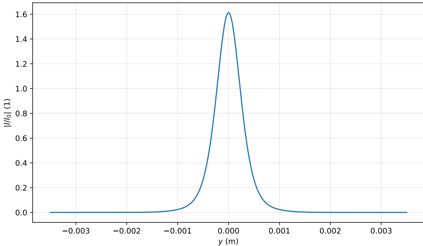
Intensity profile I(x=0, y, z=1.751)/I_0 , P_{in}=0.9P_{cr} , artificial time
